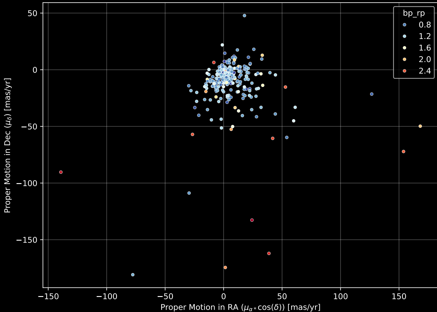
APOGEE DR17 Field: [sgr_tidal4] Proper Motion Diagram (n= 288)
