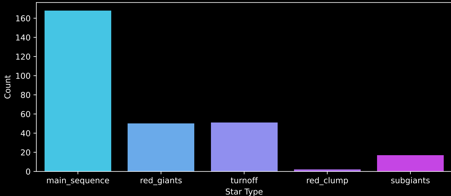
APOGEE DR17 Field: [sgr_tidal4] Count plot of Star Type
