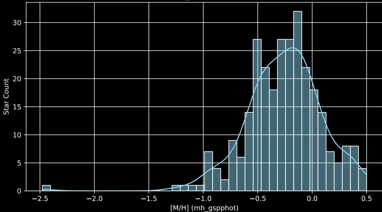
APOGEE DR17 Field: [sgr_tidal4 [M/H] (mh_gspphot) (n= 286)
