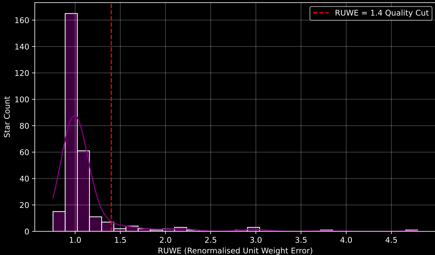
GAPOGEE DR17 Field [sgr_tidal4] RUWE Distribution (n= 280)
