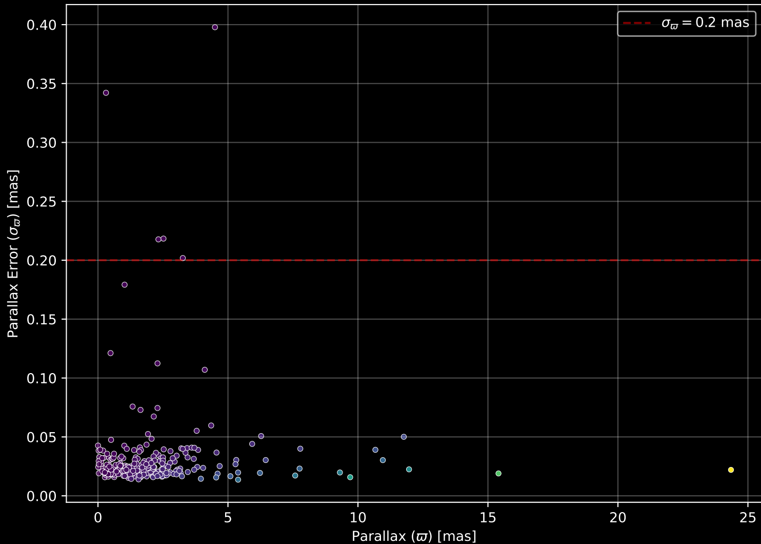
APOGEE DR17 Field: [sgr_tidal4] Parallax Quality (n= 288)
