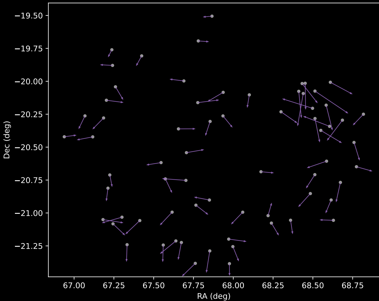
APOGEE DR17 Cluster 8 Proper Motion Vectors (n=67)
